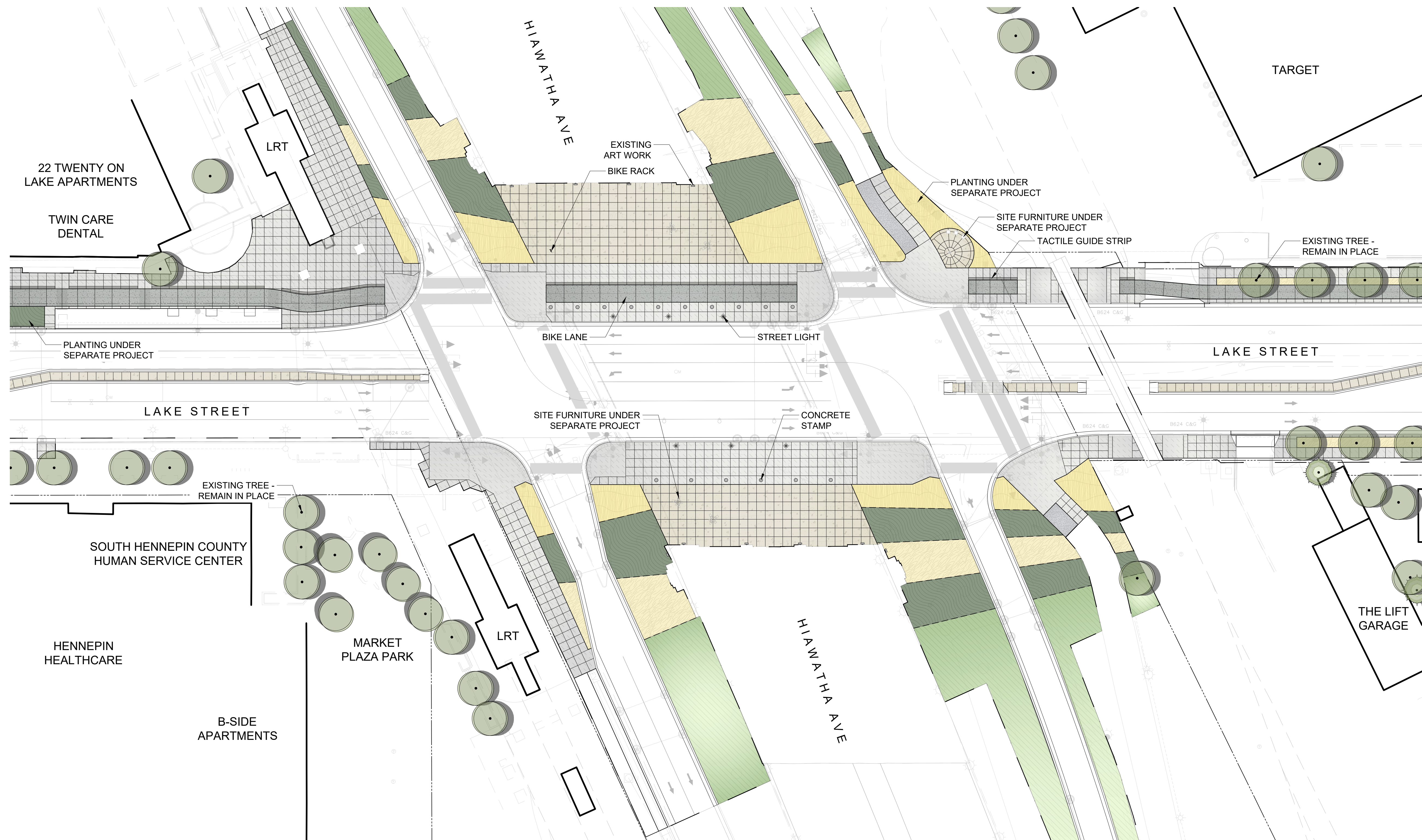
HI-LAKE INTERCHANGE ILLUSTRATIVE PLAN - 1:30 SCALE 12.06.2023
